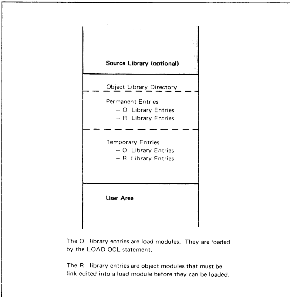
Figure 2. Format of Object Library
