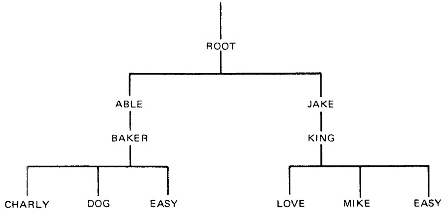
Figure 13. Calling Tree-structure of Modules Linked in Examples 8-11
